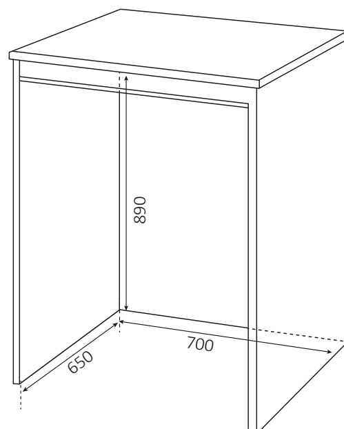
Misure interne del mobile Internal dimensions
